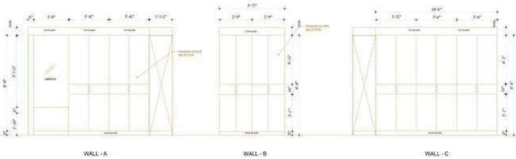
Wardrobe shutter and details
