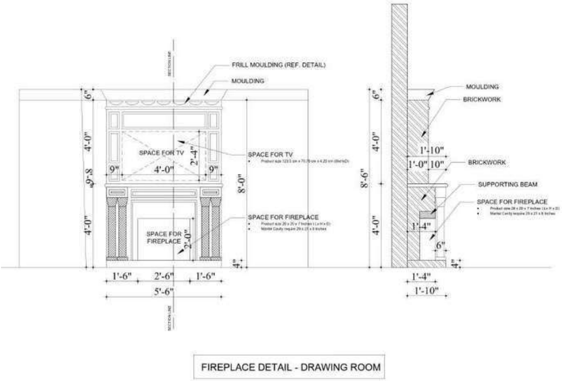
Fire place Elevation
