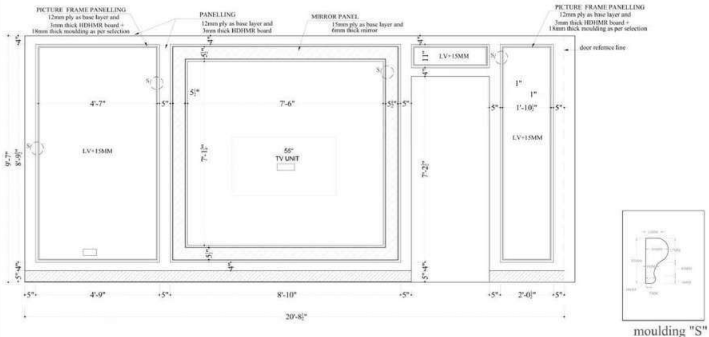
Tv wall detail
